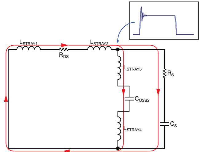
Figure 8. Snubber Circuit
