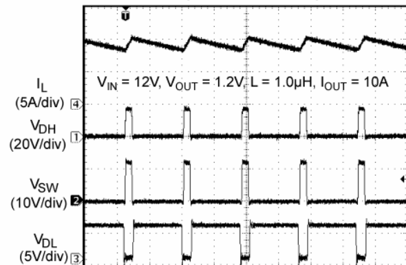
Switching Waveform (Continuous Mode)
