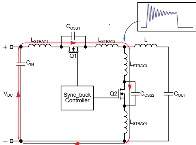
Figure 7. Output Parasitics
